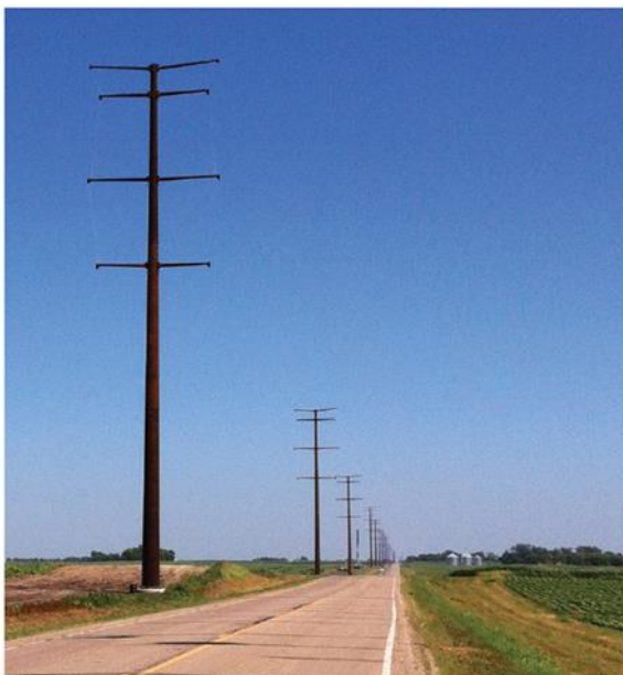
Single pole steel structures will primarily be used to reduce land impacts; some locations may require two pole structures. Poles are between 140 and 170 feet tall and will be about 1,000 feet apart. Typically, a 150-foot wide right-of-way will be required.
