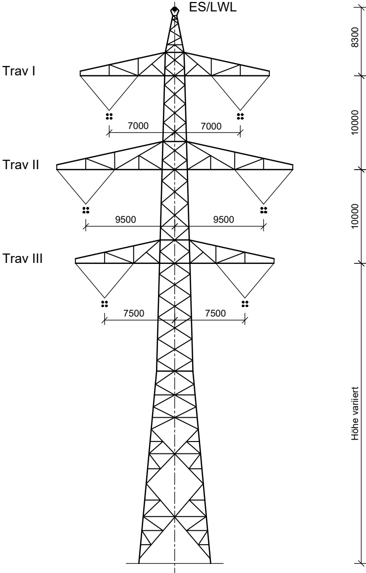
Tragmast T1; D-2-T Ltg. Nr. B161: Mast-Nr. 21, 22, 23, 24, 26, 27, 28, 34, 35, 36
